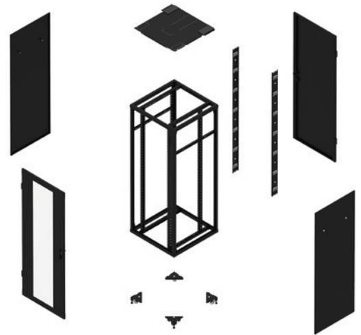
Typical 800mm wide RA Series Basic Rack Configuration
